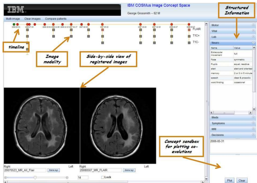
Fig. 4. User interface of COSMus. Through this interface user can access structured information obtained from various data sources at different timepoints. Also registered images can be compared with each other. Users can select concepts and their attributes and visualize their trends through time.
