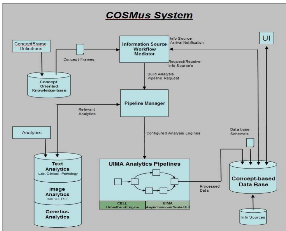
Fig. 3. The architecture of the COSMus system.
