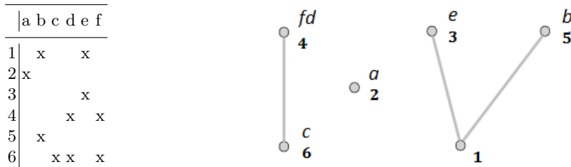
Fig. 1. A formal context with the corresponding GSH diagram.
