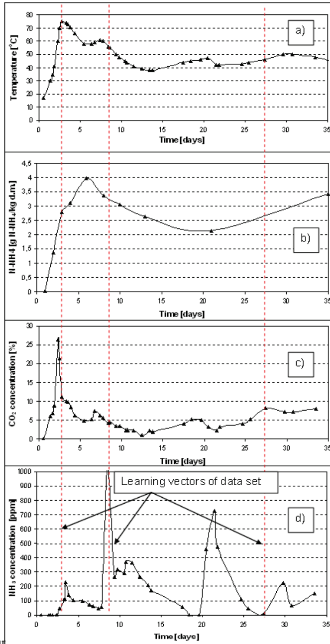
Fig. 2. Measurement of temperature changes b) Changes of ammonia nitrogen c) Carbon dioxide concentration d) Ammonia concentration; Three vertical lines are the examples of learning data vectors.
