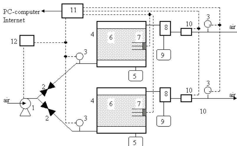
Fig. 1. Schematic diagram of the bioreactor: 1. pump, 2. flow regulator, 3. flow meter 4. isolated chamber, 5. drained liquids container, 6. composted mass, 7. sensors set, 8. air cooling system, 9. condensates container, 10. column of gases content analysis ( \text{NH}_3 , \text{O}_2/\text{CO}_2 , \text{CH}_4 ), 11. 16-channel recorder, 12. air pump steering system
