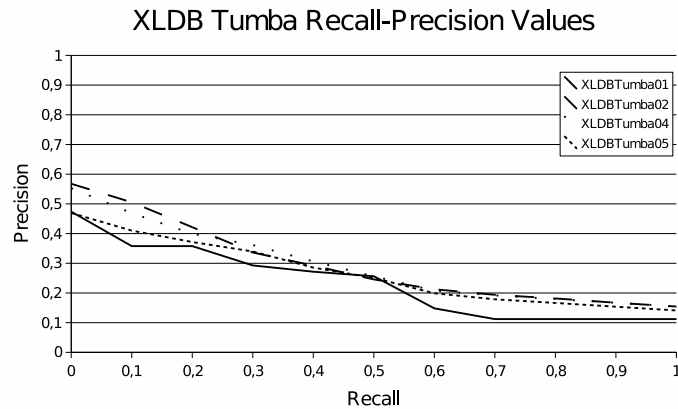
Figure 2: Recall-Precision Values for our runs, according to CLEF results.
