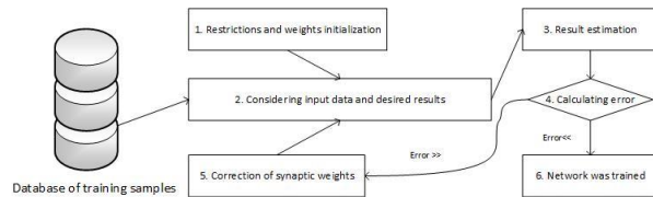
Figure 1: Functional scheme of backpropagation algorithm
