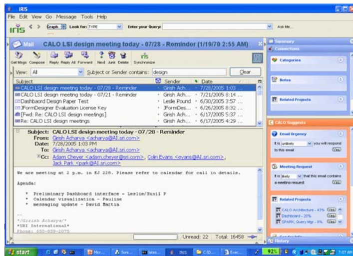
Figure 3: In the “CALO Suggests” pane, learned hypotheses about an email are presented, including reply urgency, meeting detection, project association, and others. The user can provide feedback about the system's choices, and the system will adapt accordingly.
