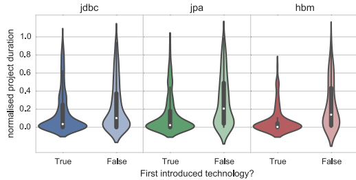
Figure 2: Violin plot (using a kernel density estimate) of the distribution of the introduction time of a technology in the Java project corpus.
