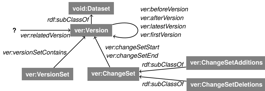
Fig. 4: Overview of the classes and properties in the version vocabulary.
