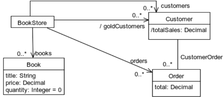
Fig. 2. The UML class diagram [23] for the CML model listed in figure 1.
