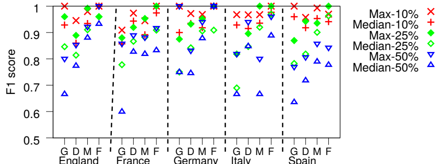
Fig. 2. F1 scores of the top-X player sets (X=10, 25, 50%) of each position and league.
