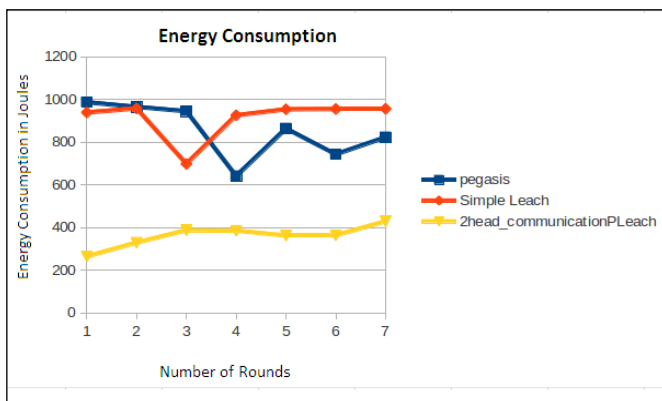
Fig. 4. Energy consumption in proposed method.
