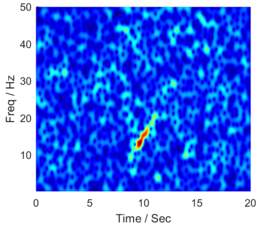
Fig. 4. Time-frequency representation for chirp signal in noise, SNR=2.
