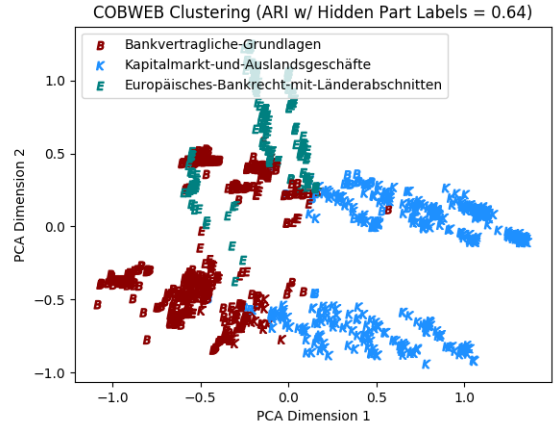
Figure 5: COBWEB clustering with p=2 , i=1149 and the ARI evaluation [HA85]
