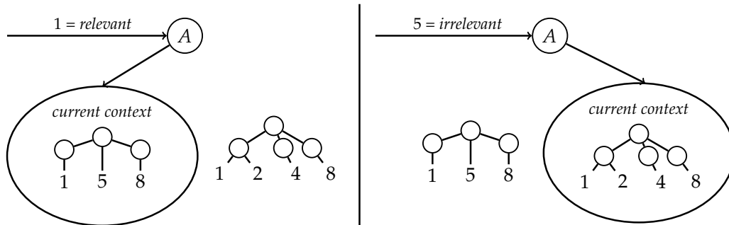
Figure 3: Incorporating user feedback in a cluster of concept hierarchies with an adaptation function (A) between the resulting clustering and class label partitions. Santos and Embrechts suggest using the ARI for supervised multilabel classification evaluation due to its ability to measure the relationship of two elements instead of the correct class label assignment [SE09]. While we only use one book, we expect an ARI above 0.5 because each chapter contains unique themes and possible overlaps in cited regulations REG . Having heterogeneous ontology clusters, an automatic merging criterion can be applied to achieve clusters of topically related concept hierarchies. Based on the ARI, this merging criterion has been implemented by Pavan et al. to extend k-means clustering [PARR11].
