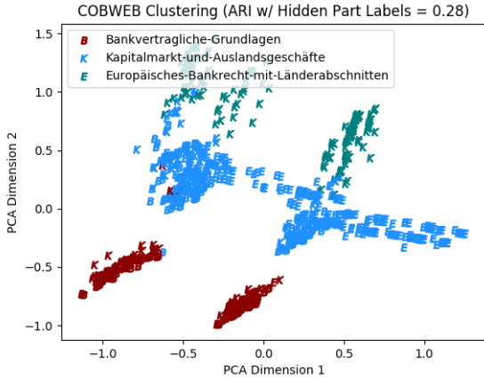
Figure 4: COBWEB clustering with p=2 , i=1020 and the ARI evaluation [HA85]
