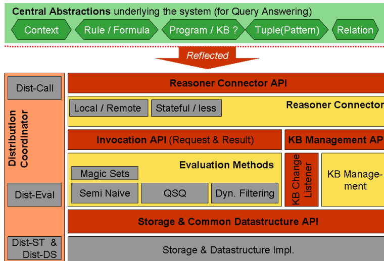
Figure 1: IRIS Architecture
