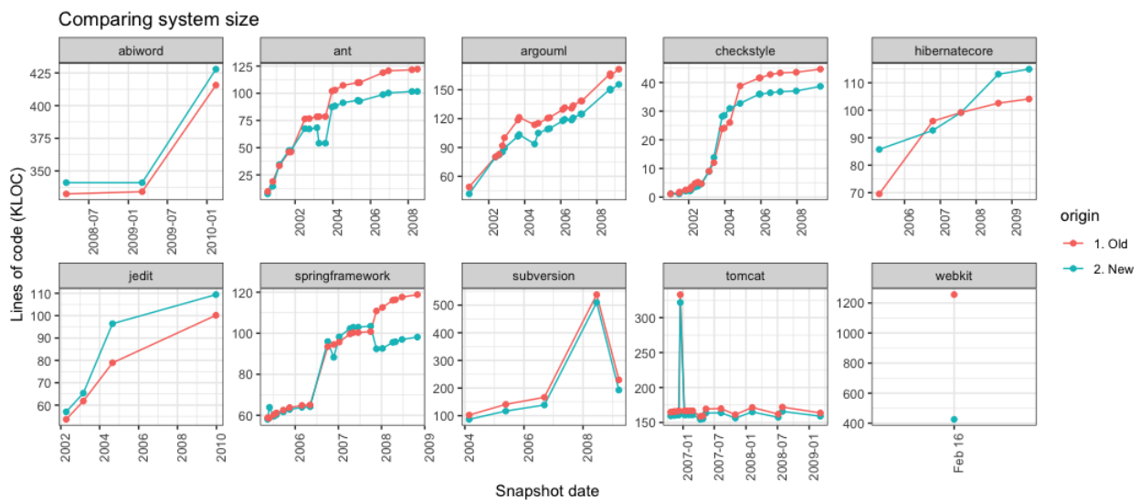
Figure 2: Comparing system sizes per snapshot (KLOC). Each point represents a snapshot of the given system, ordered by increasing date. Each snapshot is represented by two points, size in KLOC as found by Bijlsma (Red) and us (Blue).
