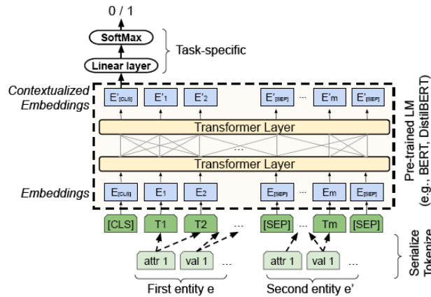
Fig. 5. Framework of the DITTO model used in our system.
