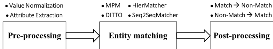
Fig. 1. Overview of our proposed system.
