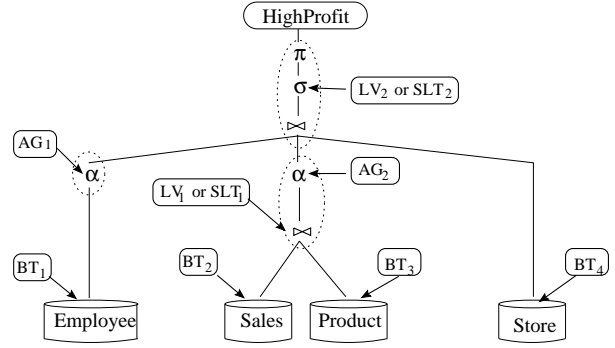
Figure 3: Possible auxiliary views for HighProfit
