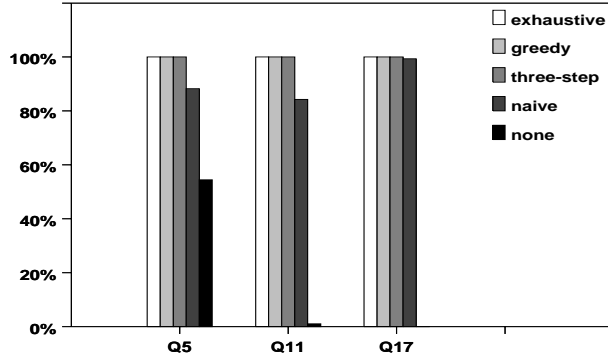
Figure 7: Optimality for TPC-D views
