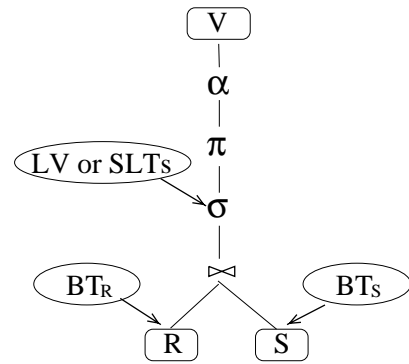
Figure 15: View structure used for v_8 and v_9
