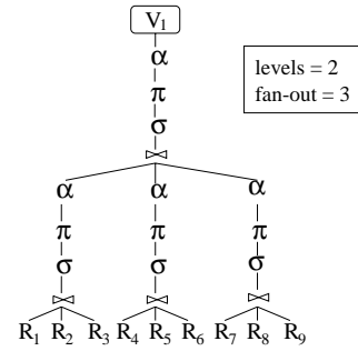
Figure 9: Structure of view v_1
