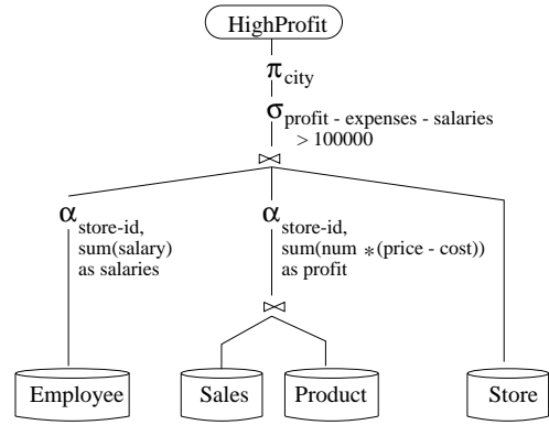
Figure 2: Normal form for HighProfit
