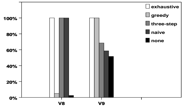
Figure 16: Optimality for v_8 and v_9
