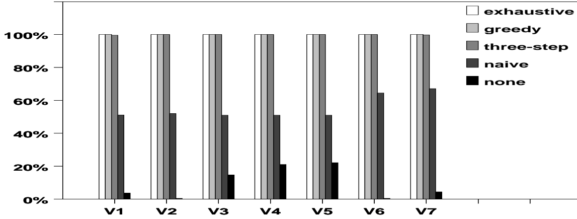
Figure 11: Optimality for synthetic views
