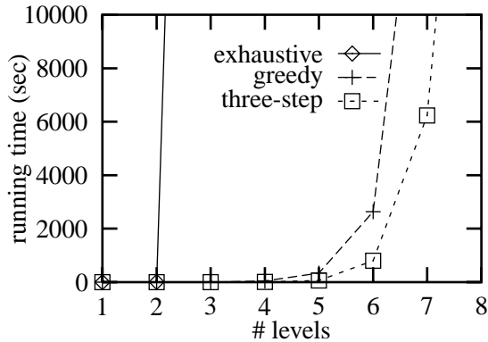
Figure 14: Running time vs. # levels
