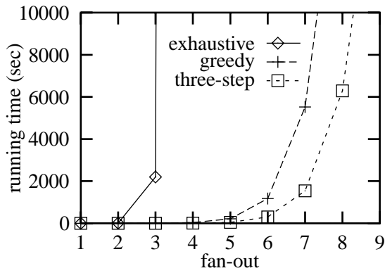
Figure 13: Running time vs. fan-out
