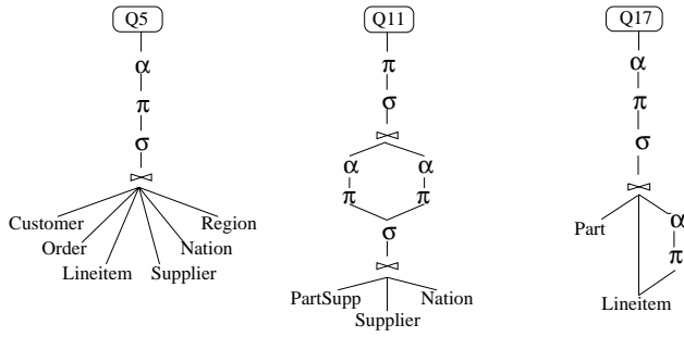
Figure 6: Materialized views for TPC-D experiments
