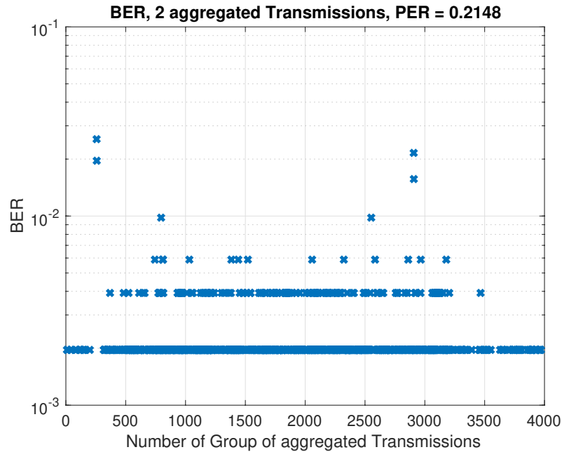
Fig. 5. BER for coherently aggregated packets (consisting of two coherently combined observations), Scenario 2, mean SNR \approx 8.1 dB.
