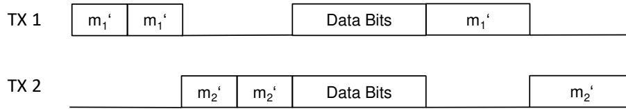
Fig. 3. Burst Structure: "Staggered".
