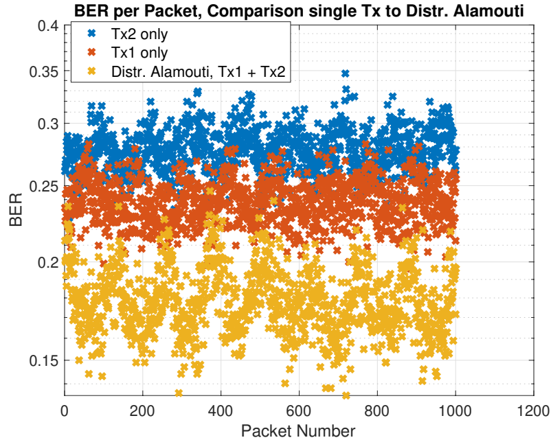
Fig. 6. BER for each of 1001 transmitted packets, Scenario 3, low SNR.
