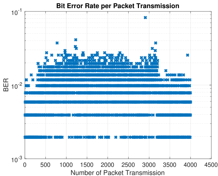
Fig. 4. BER for each of 4001 transmitted packets, Scenario 1, mean SNR \approx 8.1dB.
