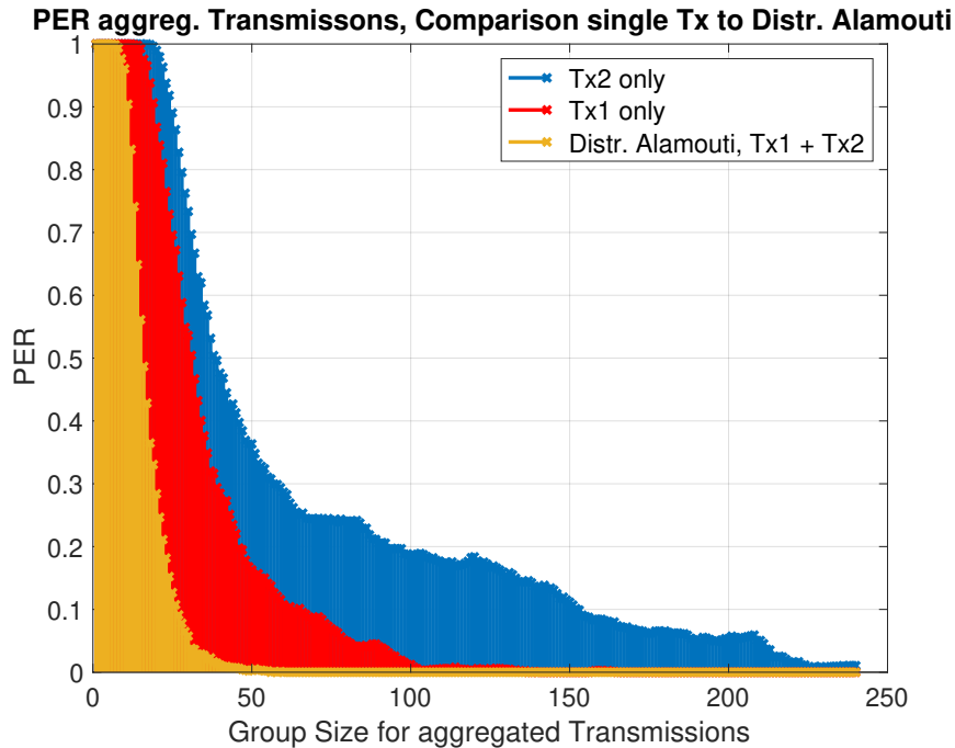
Fig. 7. PER vs. number of coherently combined packets; low SNR case.
