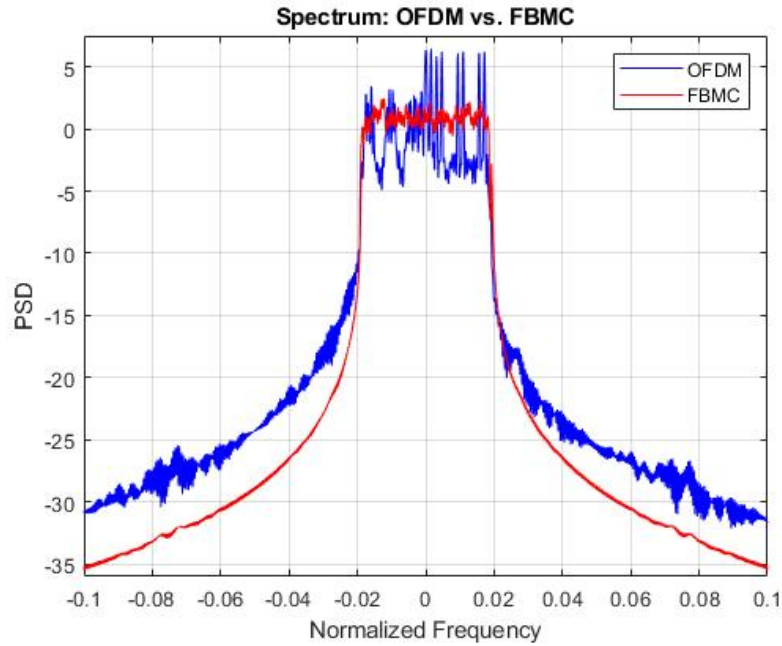
Fig. 8. Comparison between the OFDM and FBMC Spectrum.
