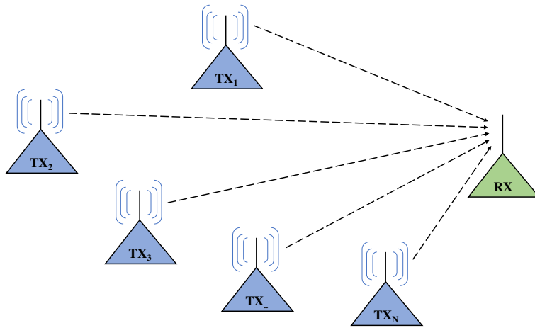
Fig. 1. System model for the demonstration system.
