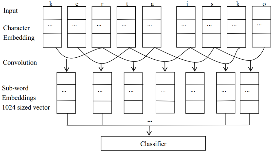
Figure 1: The sub-word level representations through 1-D convolutions on the character
