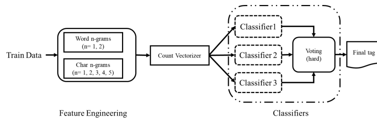
Figure 2: Architecture of ensemble of ML models.
