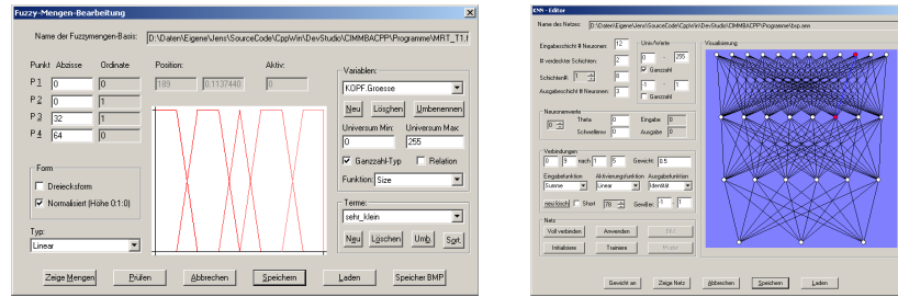
(a) Fuzzy-Editor
