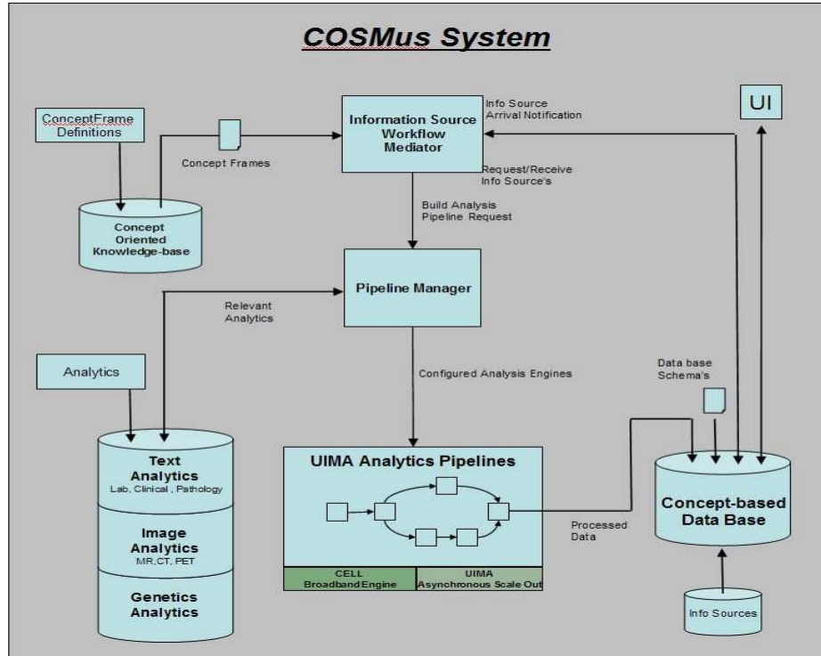
Fig. 3. The architecture of the COSMus system.
