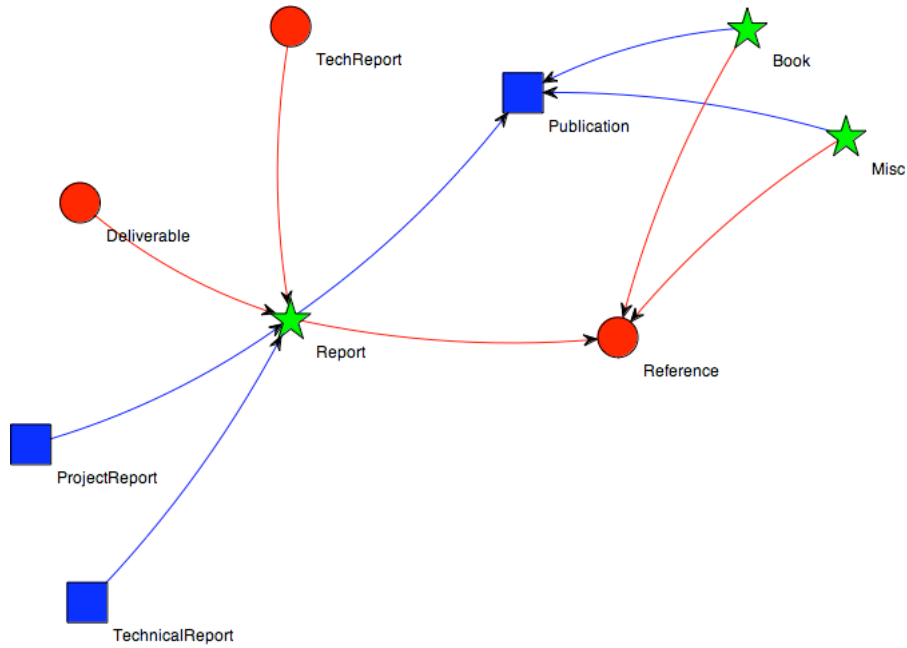
Fig. 4. Pattern 1 example and simplified visualization of the mapping between the SWRC ontology and the \langle \textit{Deliverable}, \textit{subclassOf}, \textit{Report} \rangle statement.
