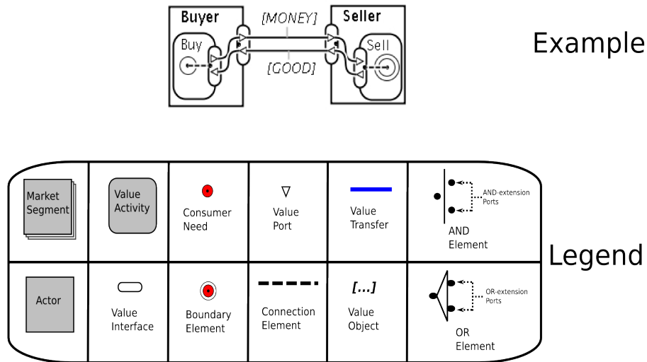
Fig. 2: e^3 value constructs for value modelling.
