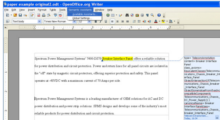
Fig. 2 Annotation of text with Equivalent Class Axioms using the Semantic Assistant
