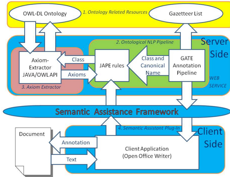
Fig. 1. Semantic Assistant Framework
