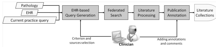
Fig. 1. Method's architecture
