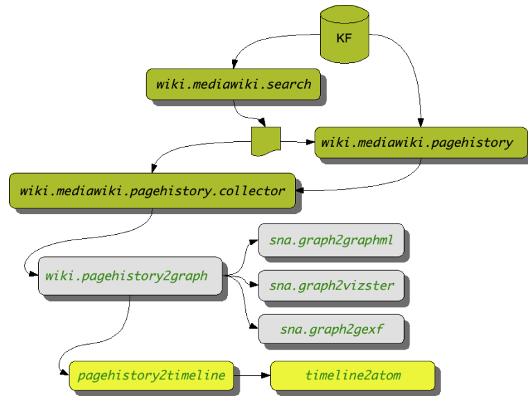
Fig. 2. Core components for collecting and processing wiki contributor data
