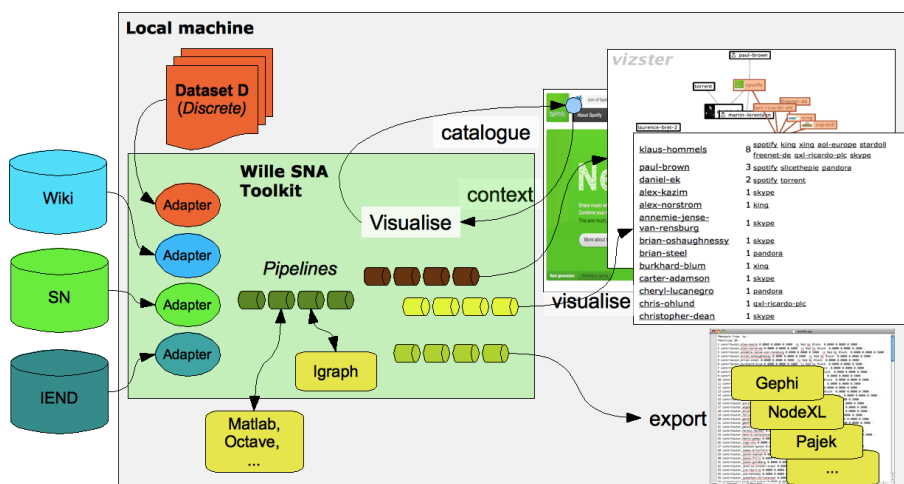
Fig. 1. Data-driven visual SNA with Ville
