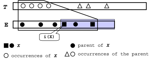
Figure 1: An example of the parent of X : The parent of X is obtained by deleting items larger than i(X) (in the grey area) and take a closure.
