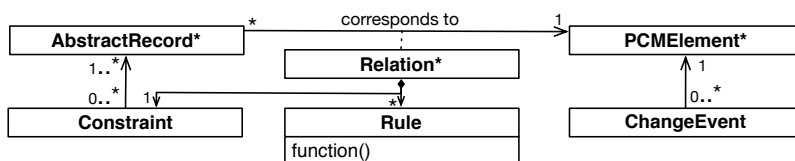
Fig. 2. The Run-Time Architecture Correspondence Meta-Model.
