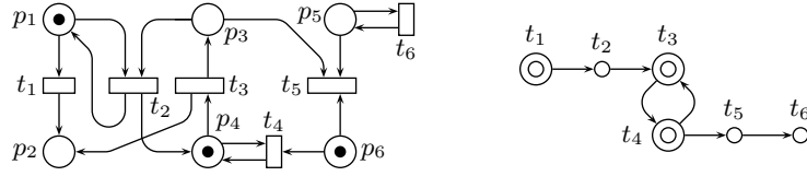
Fig. 1. A marked Petri net and its “ \sim_M ”-graph, with p_{t_5} = p_5 .
