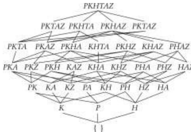
Fig. 1. A simple Hasse diagram
