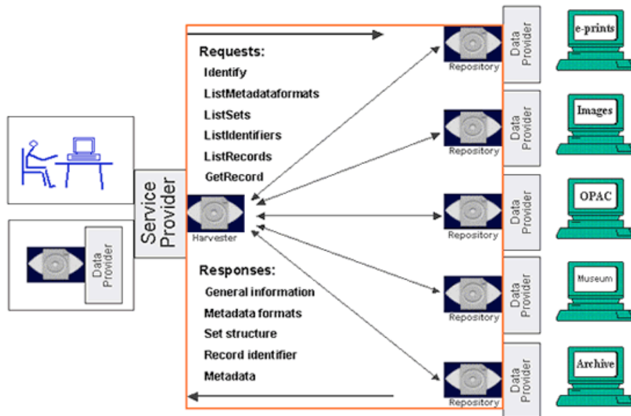
Fig. 1. OAI-PMH structure-model
