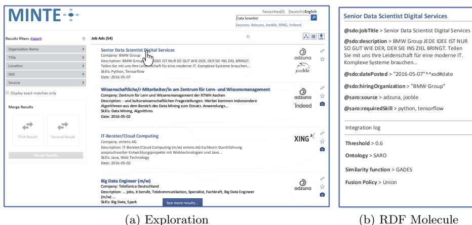
Fig. 2: MINTE + in the Job Market Analysis application. (a) A faceted browser user interface allows to search and analyze the data scientist job market in Europe. (b) The integration log shows configuration of the integration process.
