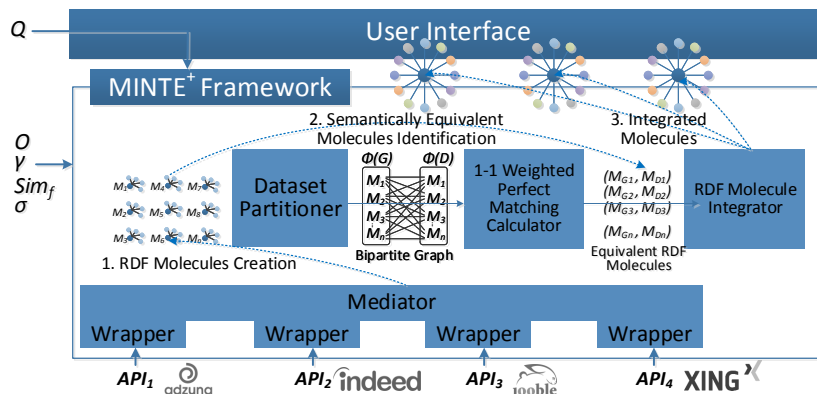
Fig. 1: MINTE+ Architecture. Data from web sources, e.g., Adzuna, Indeed, Jooble, and XING is collected to answer a keyword query Q . A mediator creates RDF molecules from these sources; they are expressed the SARO ontology O . Dataset Partitioner builds a bipartite graph using a similarity function Sim_f , e.g., GADES and configurable threshold \sigma ; a 1-1 perfect matching to identify equivalent RDF molecules is produced. The RDF Molecule Integrator employs a union fusion policy to synthesize RDF molecules into a knowledge graph.
