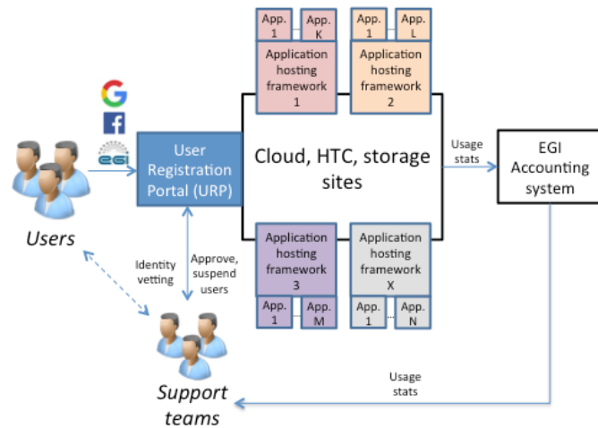
Figure 1. Infrastructure architecture
