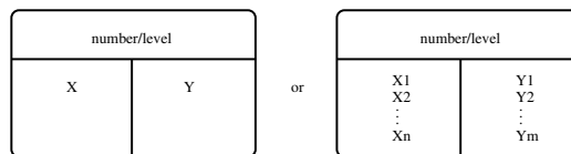
Figure 2. An ARD table: the basic scheme for X \rightarrow Y
