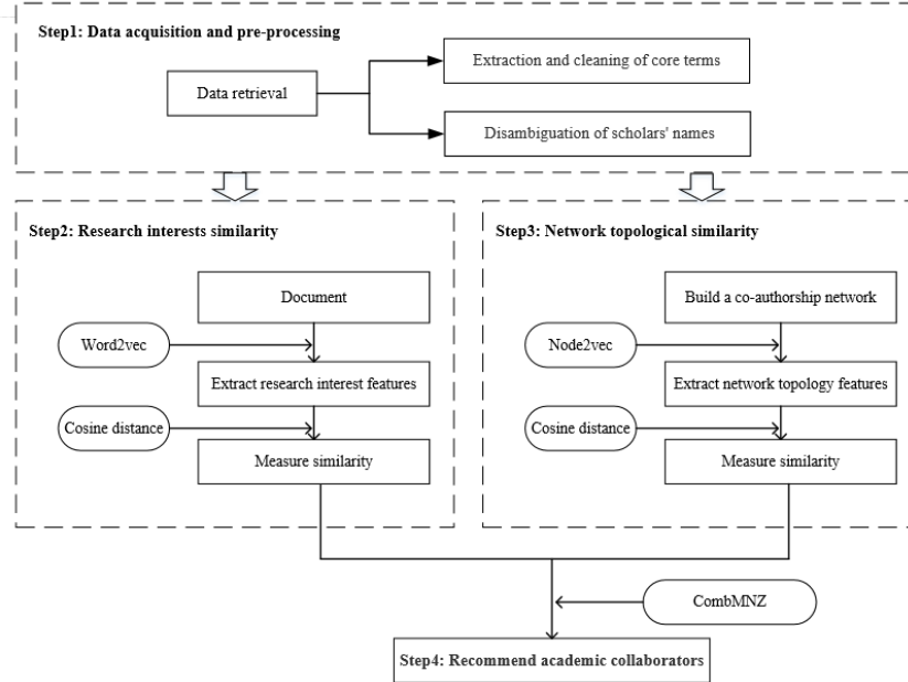
Fig. 1. Analytical framework
