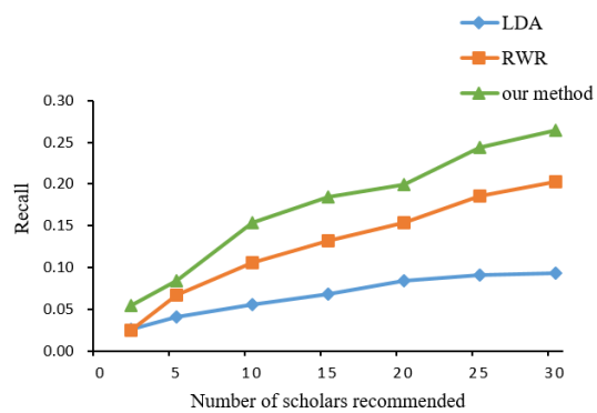
Fig. 5. Recall
