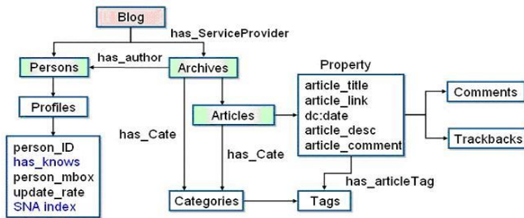
Fig. 2. The blog ontology describes the profile of a blogger with his blog articles
