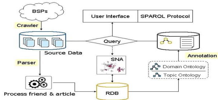
Fig. 5. The semantic social web blog portal to experiment our Web 2.0 ↔ Web 3.0 bridging model
