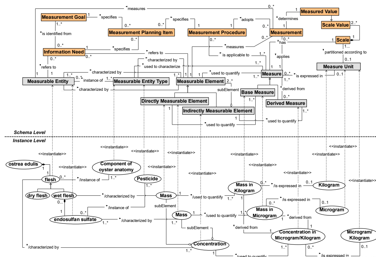
Figure 5: Extension of I-ADOPT ontology through M-OPL use
