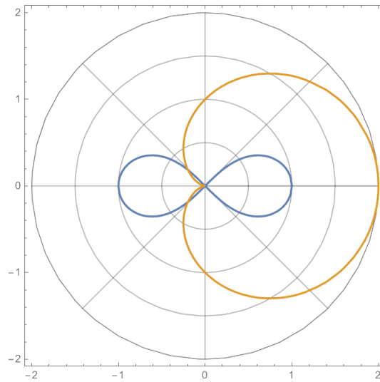
Figure 3: The plot of r^2 - \cos(2t) = 0, r - (1 + \cos(t)) = 0 .
