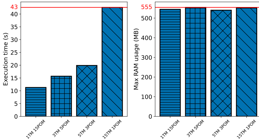
Figure 2: RMLWeaver-JS has a significant increase in execution time, at 43 seconds, for the test case with 15 triples maps and 1 predicate object map despite almost constant memory usage across the different test cases.
