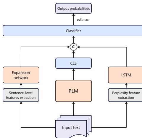
Figure 1: Our model architecture for text detection and attribution
