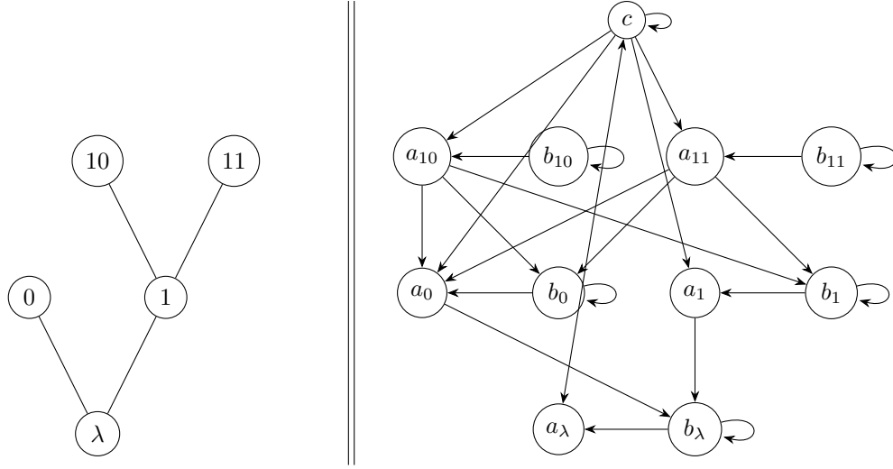
Figure 1: Example of our encoding of trees into AFs: the left-side represents the tree \{\lambda, 0, 1, 10, 11\} , the right-side is the resulting AF. When applied to trees T of infinite height, [T] will be encoded into the stable, complete, and admissible extensions of \mathcal{F}_T . For the example shown in the figure, the only admissible extension of \mathcal{F}_T is the empty one, since [T] = \emptyset .
