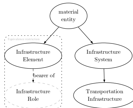
Figure 2: Common Core Ontologies infrastructure constraints. Solid arrows represent super-class relations
