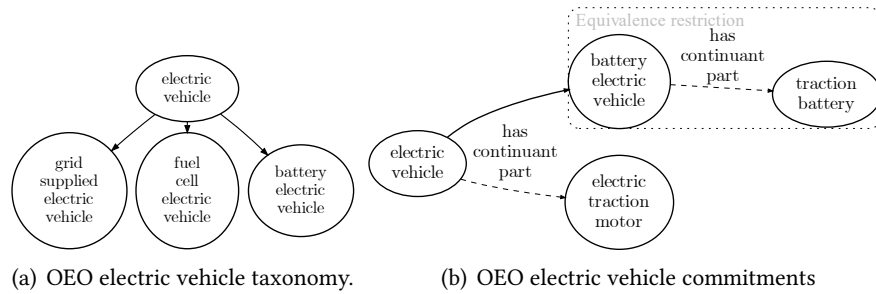
Figure 1: OEO ontological commitments relevant to the context of charging infrastructure. Note that we exclude grid related commitments, mostly because we have to properly outline a scenario to implement them. Solid arrows represent super-class relations.
