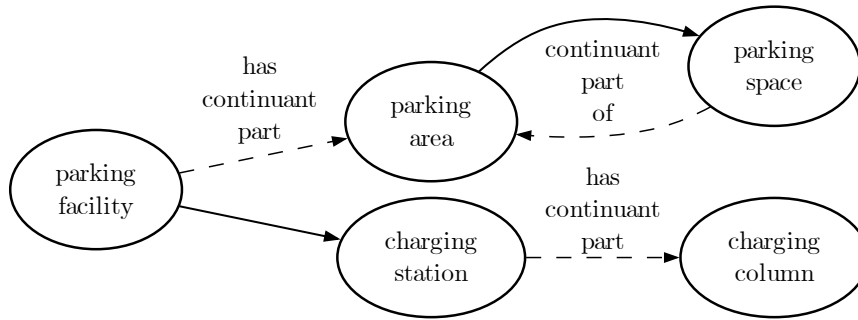
Figure 4: Parking area, place, and facility implementations in our ontology. This model builds on the taxonomy of the CCO Facility Ontology. Solid arrows represent super-class relations.
