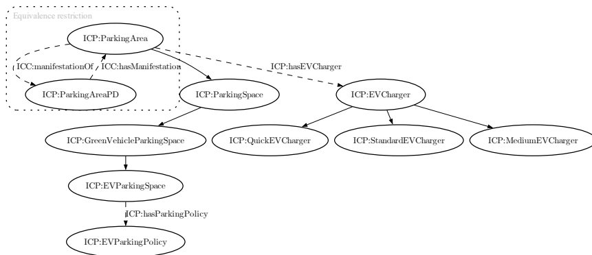
Figure 3: iCity parking ontology commitments associated with charging infrastructure. Solid arrows represent super-class relations.
