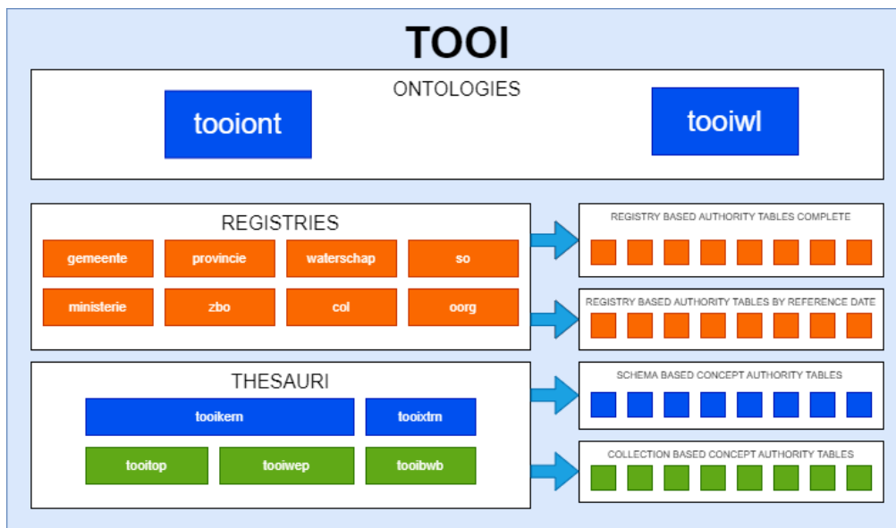
Figure 1: An overview of the TOOI modules constituting the TOOI knowledge graph.
