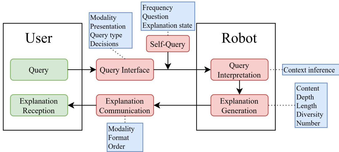
Figure 1: Our framework for the explanation process, adapted from the literature [11, 12], with possible personalisation strategies identified for each component.
