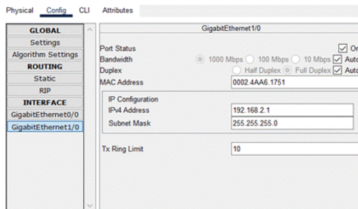
Figure 14: Office2 Node Configuration Window.
