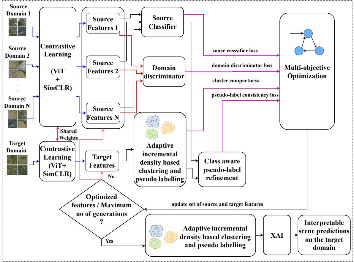
Figure 1: Proposed XMUDA-CLAC framework
