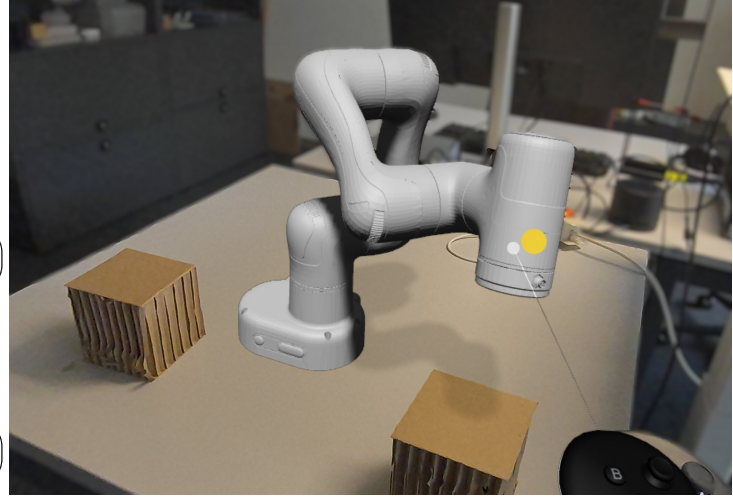
Figure 5: Mock-Up 3D view of the URDF model representing the 6-DoF robotic arm
