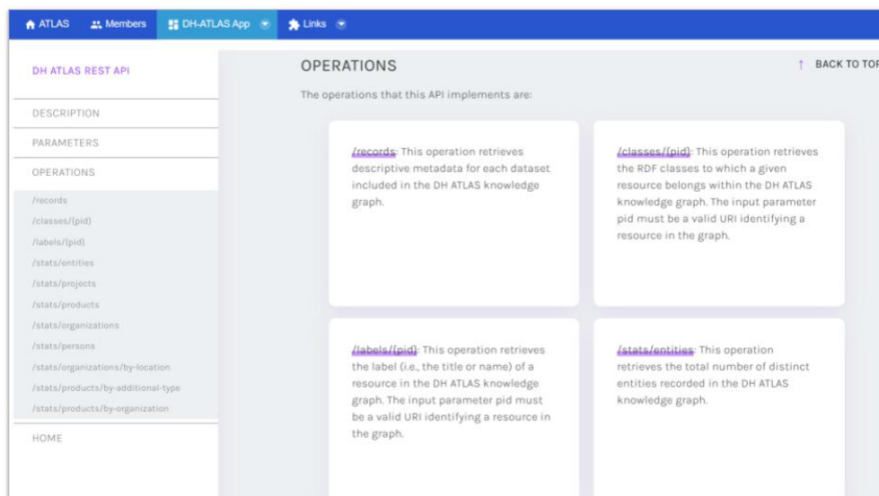
Figure 4: Figure displaying an excerpt of the RESTful API documentation made available through RAMOSE.
