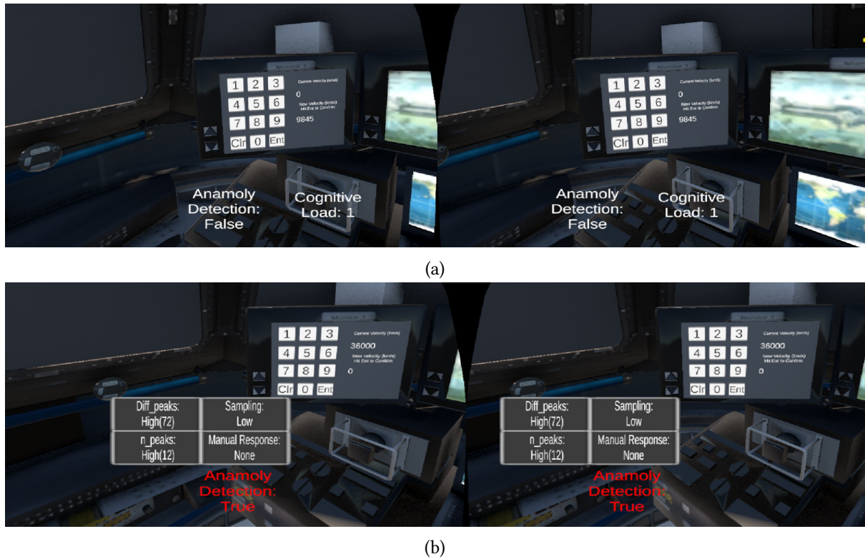
Figure 2: (a) In the first scenario, the user is interacting with the velocity setting interface in the environment while getting update of the anomaly detection and cognitive load. (b) In the case of an alert, the user can see the most important features about the anomaly and respond based on the user's analysis.
